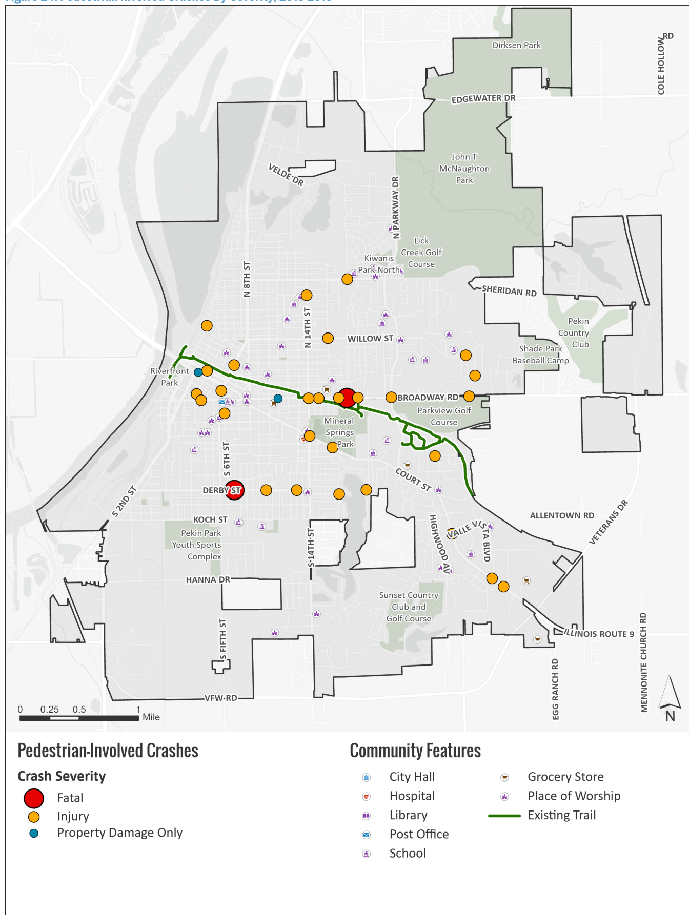
Figure 24. Pedestrian-Involved Crashes By Severity, 2015-2019
