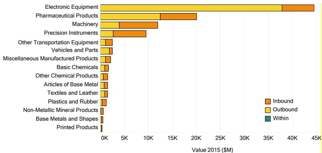
Figure 1-36: Top 15 Commodities by Value Shipped by Air, 2015
